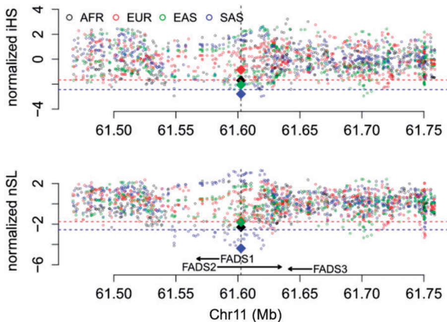
Fig. 3. Patterns of normalized iHS and nSL ( y -axes) across a 300-kb genomic region ( x -axis) around the FADS gene cluster in four continental regions, each combining multiple populations in the same region. The two statistics were calculated for each of the common SNPs (minor allele frequency >5\% ) in the genomic region, as well as for the rs66698963 indel. The position of rs66698963 is indicated as a vertical black dashed line. The values for rs66698963 in each continental region are highlighted as diamonds filled with region-specific colors. The red dashed lines represent empirical P values of 0.05, while the blue dashed lines represent empirical P values of 0.01 based on estimates in the SAS continental region. Note that the statistical cutoffs vary slightly in different continental regions. Detailed representations for each continental region with their specific significant cutoffs are presented in supplementary figs. S13–S16, Supplementary Material online .
